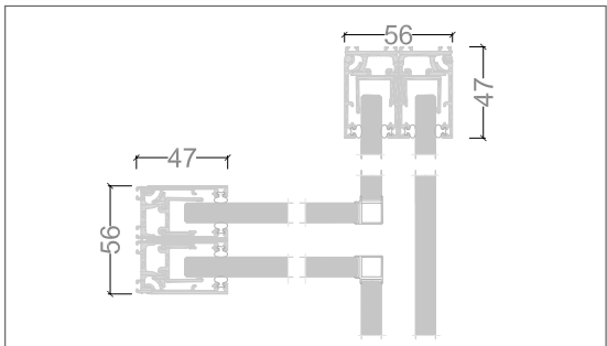
"T" JUNCTION
