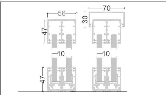
VERTICAL SECTION
