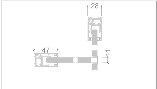
"T" JUNCTION
