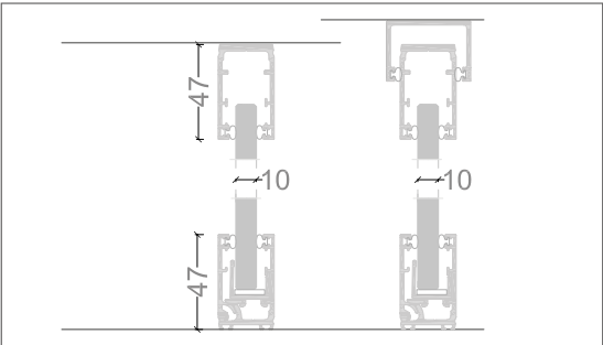
VERTICAL SECTION
